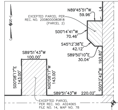
DETAIL "A" 1" = 100'
